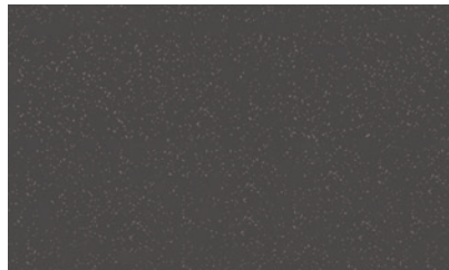
Graphite (Metallic)
